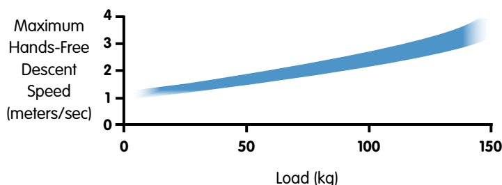
DEUS 3200 Maximum Hands-Free Descent Speed is Dependent on Load
